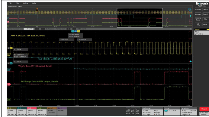
Figure 13: SDATA setup time before BCK rising edge (Data 1)
