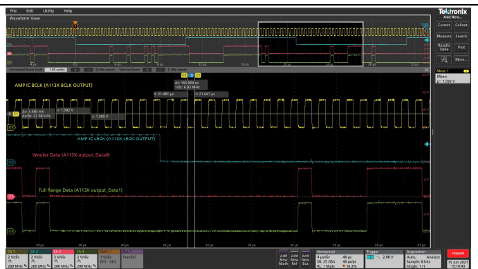
Figure 8: Hold time of Din
