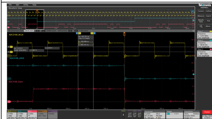
Figure 15: WCK setup time before BCK rising edge
