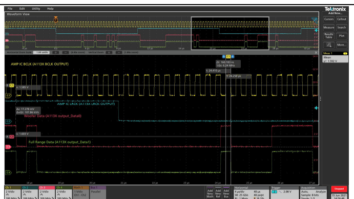
Figure 10: BCK low time
