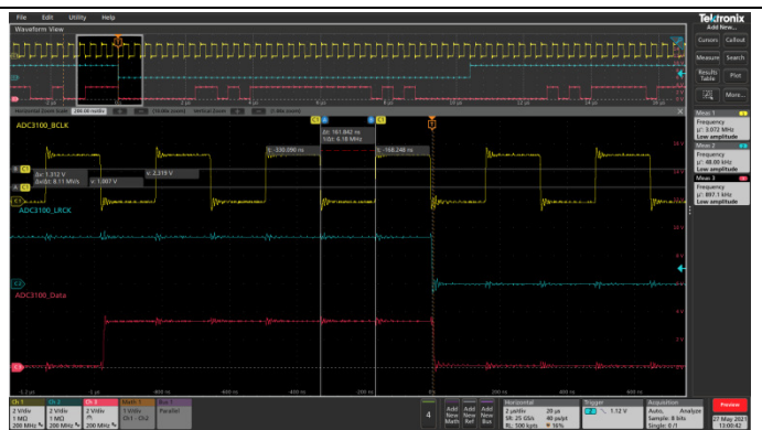
Figure 16: BCK rising edge before WCK edge
