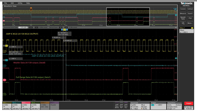
Figure 14: SDATA hold time after BCK rising edge (Data 1)
